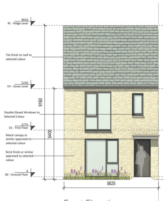
Front Elevation Character Area 1
