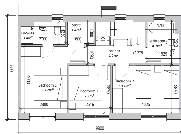
First Floor 52.7sqm
