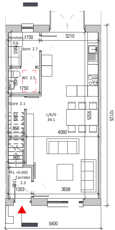
Ground Floor 47.4 sqm
