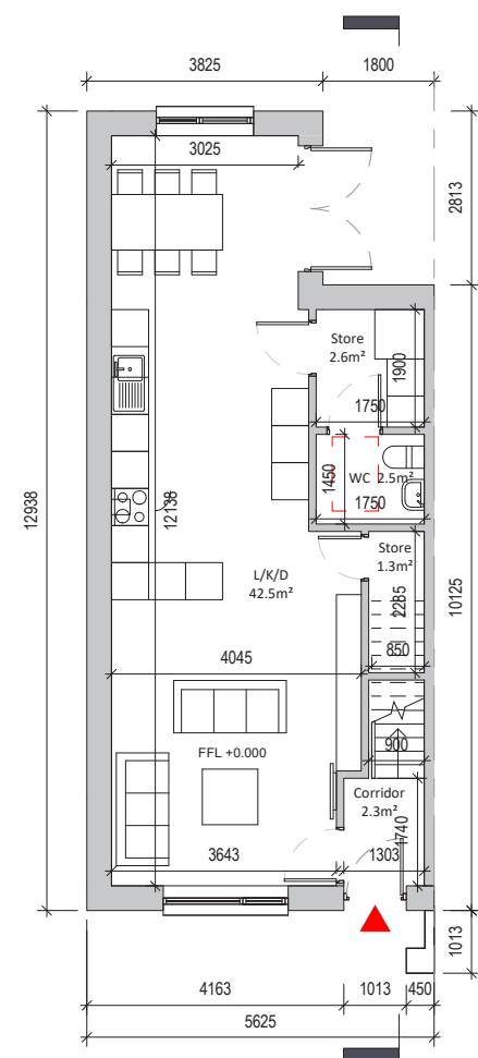
Ground Floor 55.7sqm
