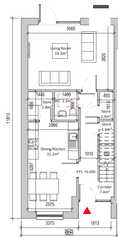
Ground Floor 53.6sqm
