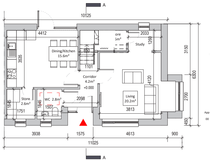
Ground Floor 50.9sqm
