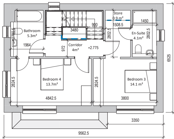
First Floor 50.2 sqm
