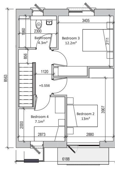
Second Floor 50.2 sqm
