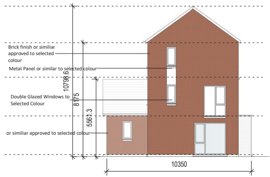
Left Elevation
