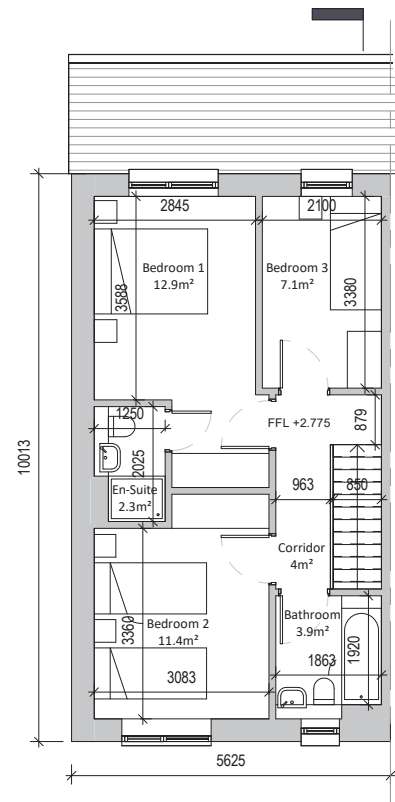
First Floor 46.7sqm
