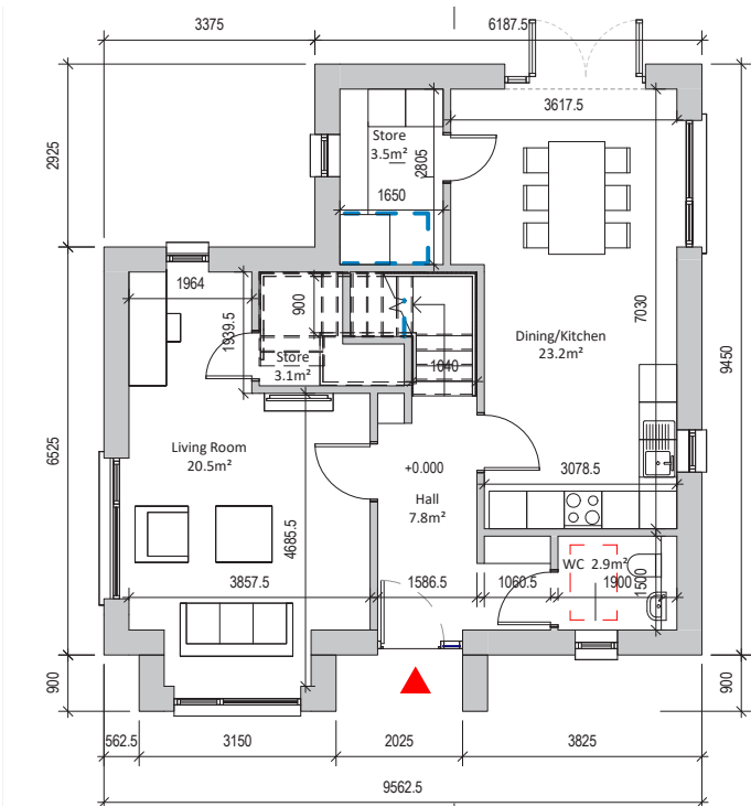
Ground Floor 68.1 sqm
