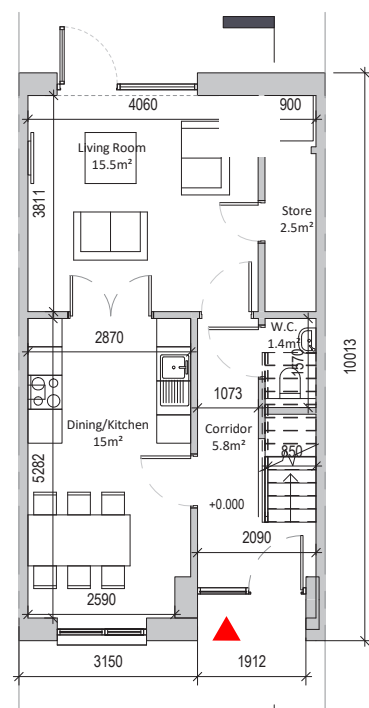
Ground Floor 44.8 sqm
