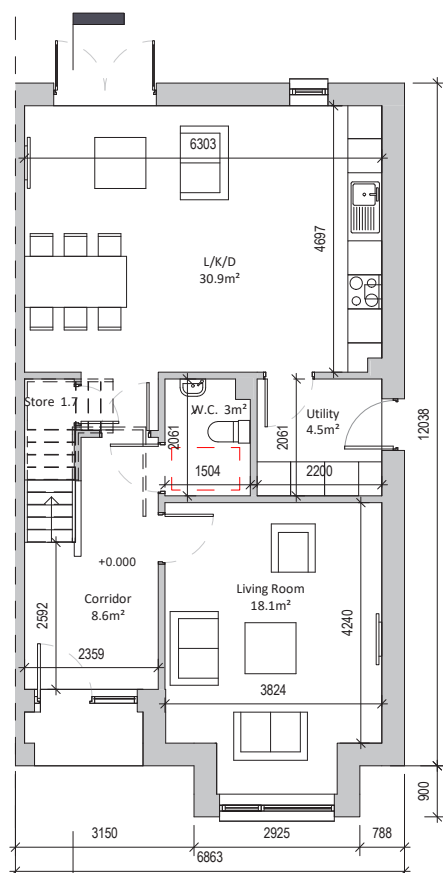
Ground Floor 70.4 sqm
