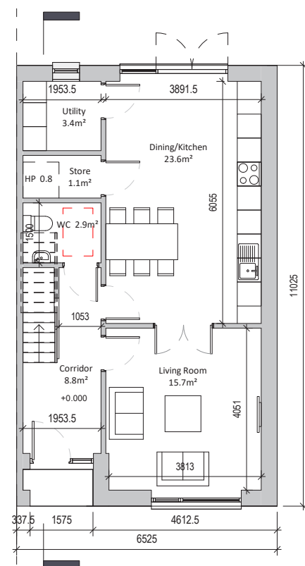
Ground Floor 59 sqm
