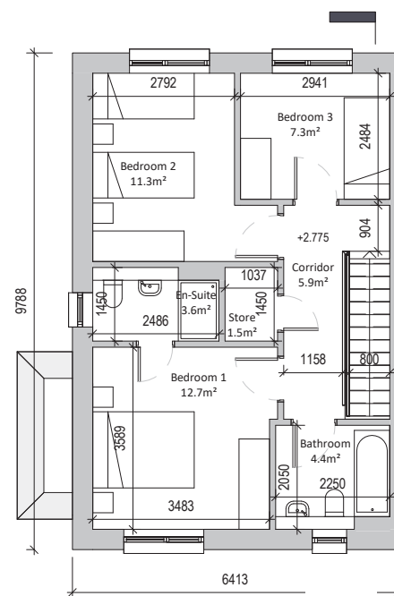
First Floor 52.6 sqm
