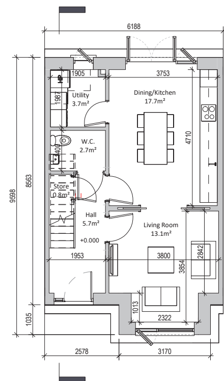
Ground Floor 70.4 sqm
