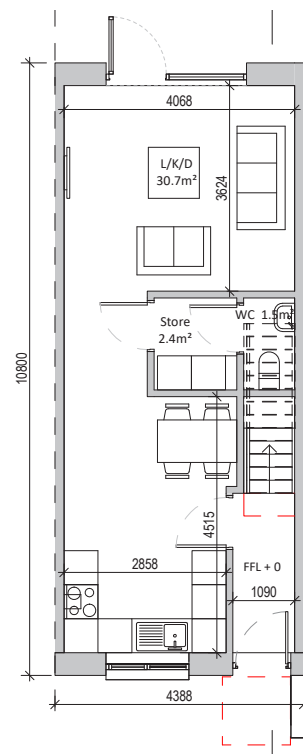
Ground Floor 40.5sqm
