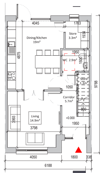
Ground Floor 50.6 sqm
