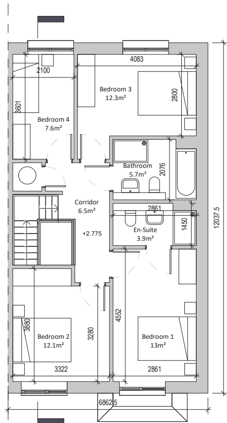
First Floor 70.8 sqm
