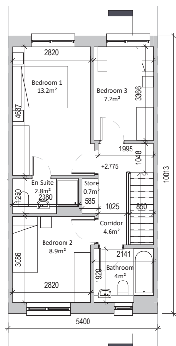
First Floor 46.7sqm
