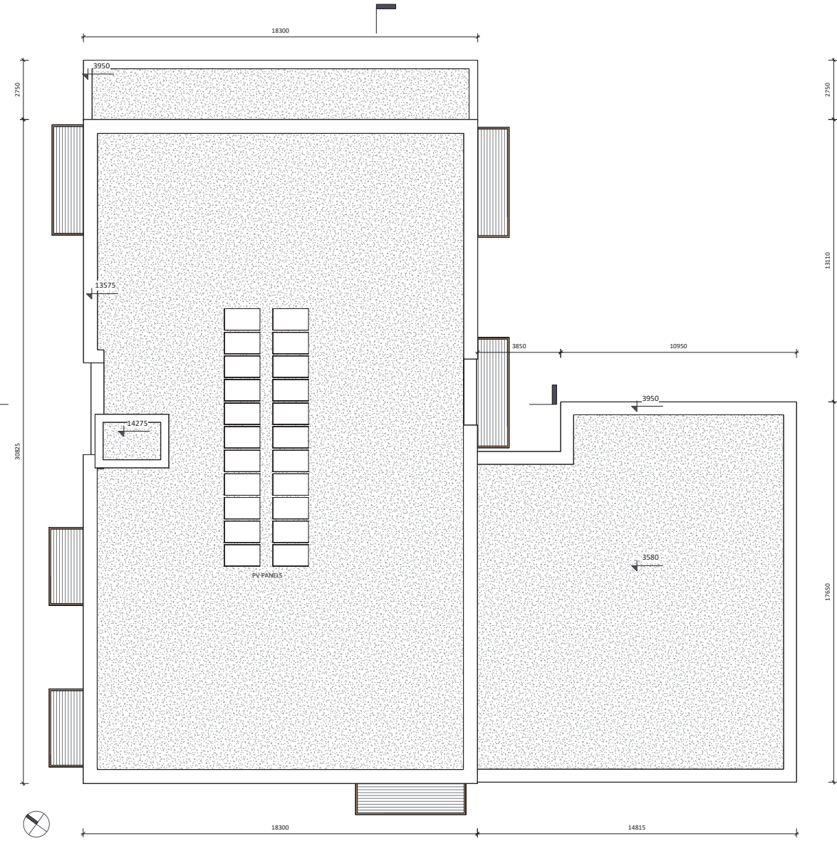
Roof Plan
