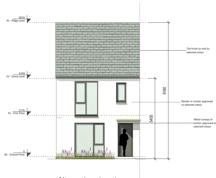
Alternative elevation (render finish)
