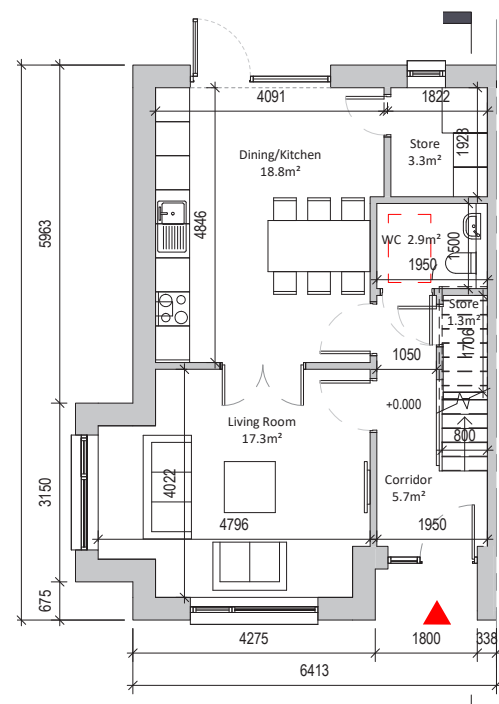
Ground Floor 52.8 sqm
