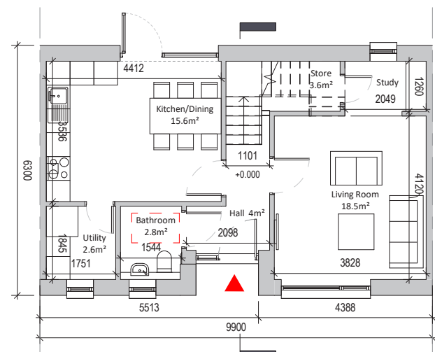
Ground Floor 50.9sqm
