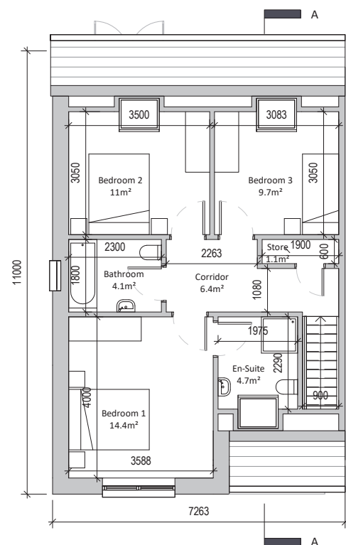
First Floor 56.7sqm
