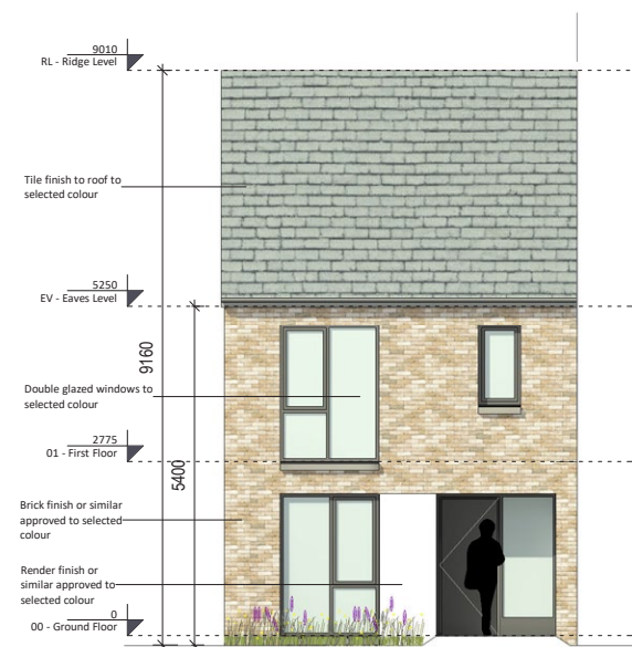
Front Elevation Character Area 2
