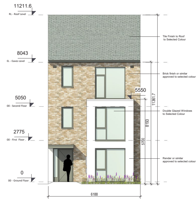
Front Elevation Character Area 2
