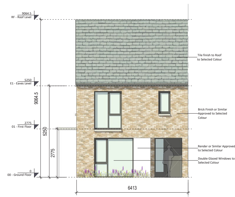
Front Elevation Character Area 2
