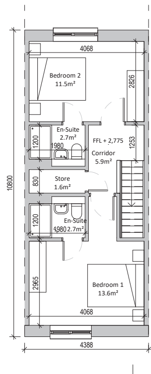
First Floor 40.5sqm
