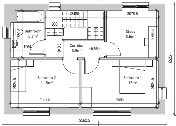
Second Floor 50.2 sqm
