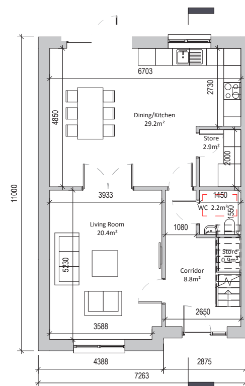
Ground Floor 67 sqm
