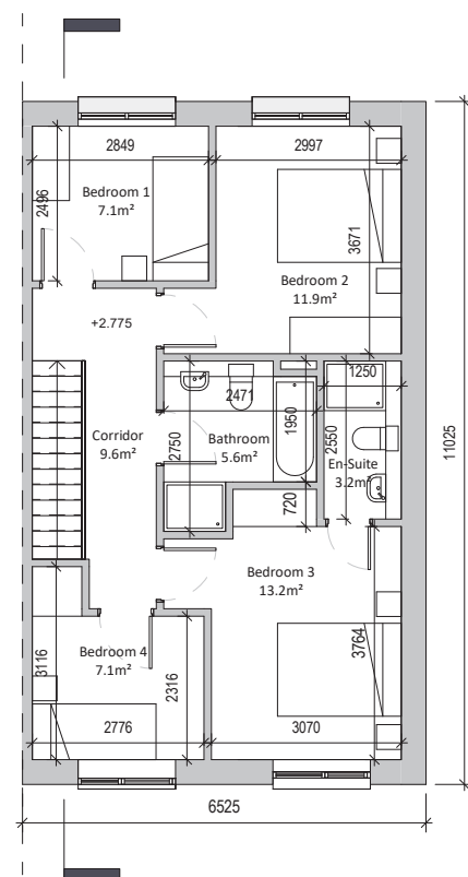
First Floor 61 sqm
