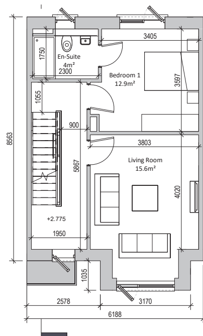
First Floor 70.8 sqm
