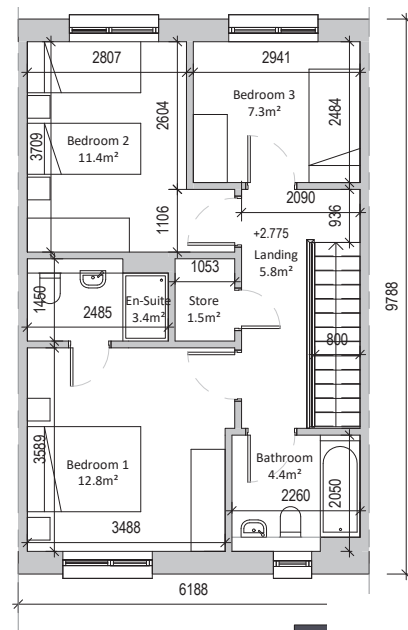
First Floor 52.7sqm
