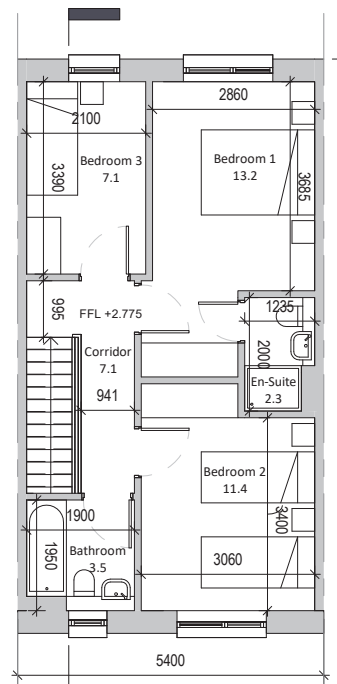
First Floor 47.4sqm
