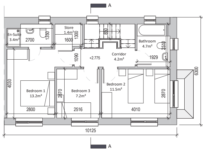
First Floor 52.7sqm
