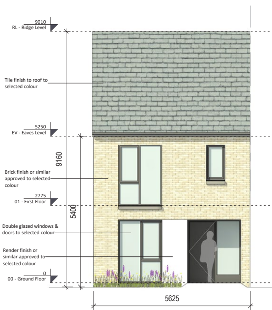
Front Elevation Character Area 1
