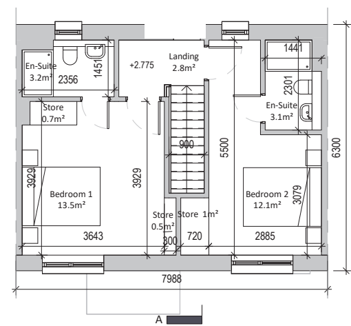
First Floor 42.1 sqm
