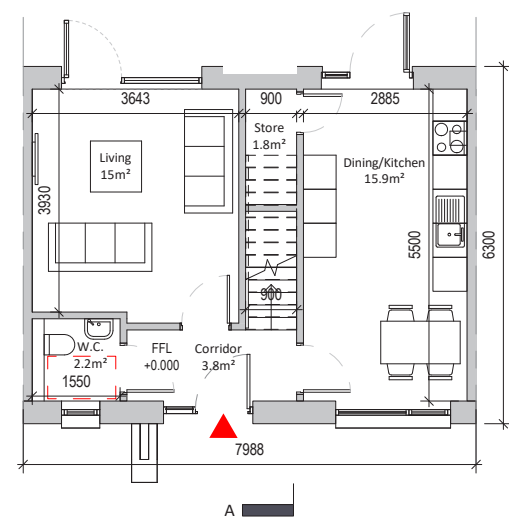
Ground Floor 42.1sqm
