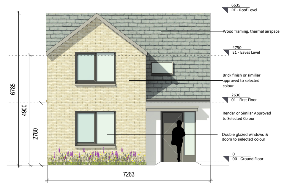
3 Front Elevation -Character Area 1 1 : 100
