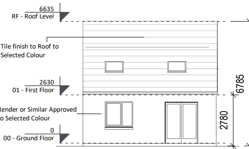
5 Rear Elevation 1 : 200
