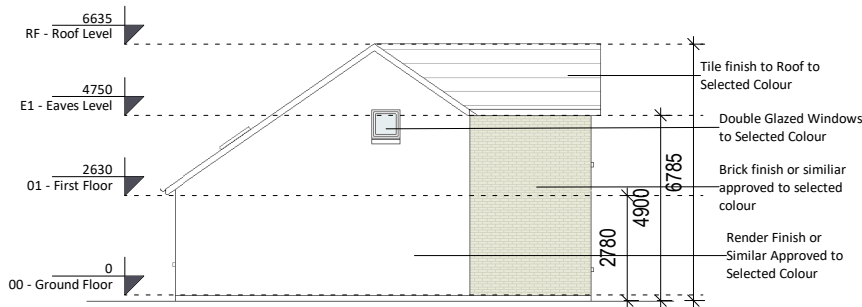
4 Left Side Elevation 1 : 200
