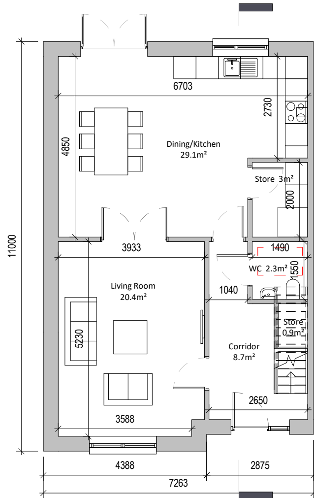
1 H3Q Ground Floor Plan 1 : 100
