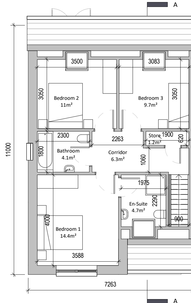
2 H3Q First Floor Plan 1 : 100
