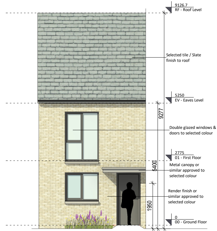
4 H2A1-Front Elevation - Character Area 1 1 : 100
