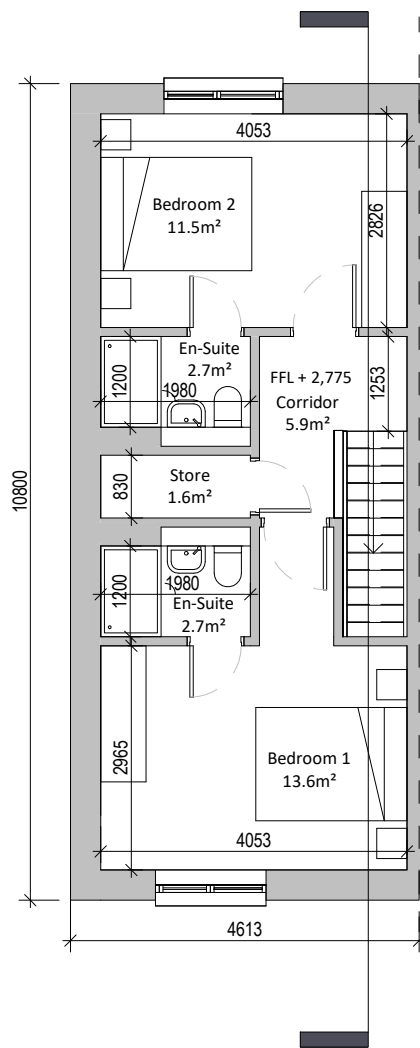
2 H2A1 First Floor Plan 1 : 100
