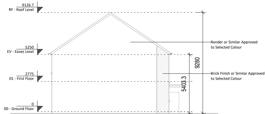
6 H2A1-Side Elevation 1 : 200
