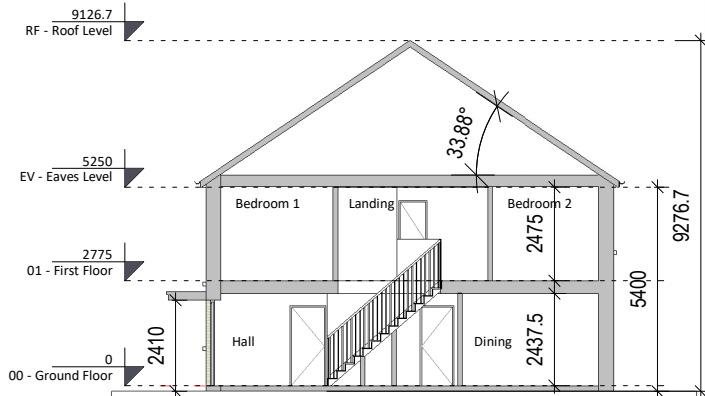
3 H2A1-Section AA 1 : 200
