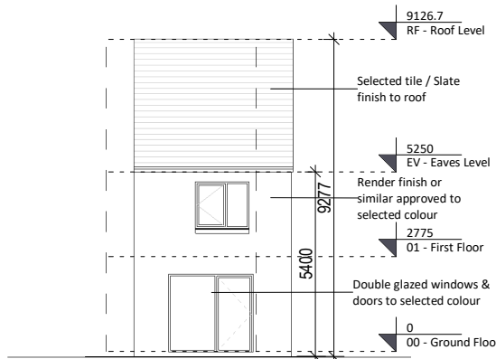
5 H2A1-Rear Elevation 1 : 200
