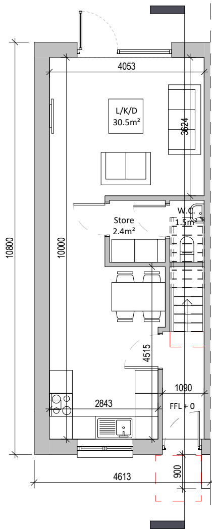
1 H2A1 Ground Floor Plan 1 : 100
